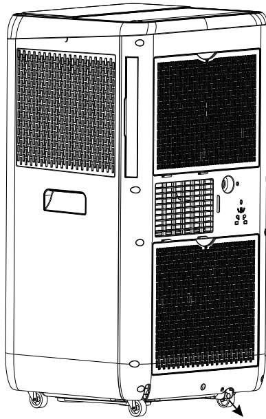
Manual drainage (Cooling and Heating)
